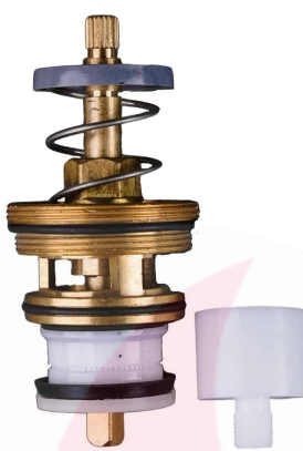
JKC PARRYWARE TYPE 40MM METROPOLE FLUSH VALVE PISTON KIT - (JKC-216-NEW)
