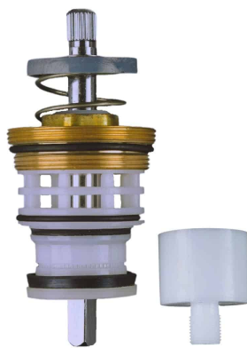
JKC MARC TYPE 40MM METROPOLE FLUSH PISTON KIT -
