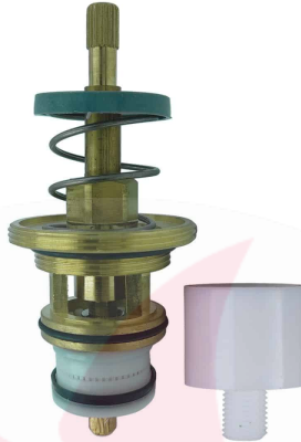
JKC PARRYWARE TYPE 32MM METROPOLE PISTON KIT - (JKC-215)
