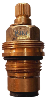
JKC PLUMBER TYPE WATER TAP SPINDLE - 1/2" (JKC-1043)
