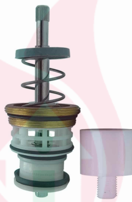
JKC JOHNSON TYPE 40MM METROPOLE FLUSH VALVE PISTON KIT - (JKC-225)
