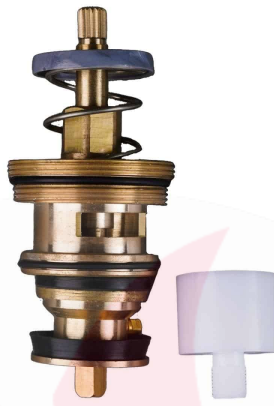
JKC PARRYWARE TYPE 40MM METROPOLE FLUSH VALVE PISTON KIT - (JKC-217-OLD)
