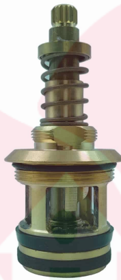
JJC ESS ESS TYPE SINGLE LEVER FLUSH FITTING - 42MM (JKC-1082)
